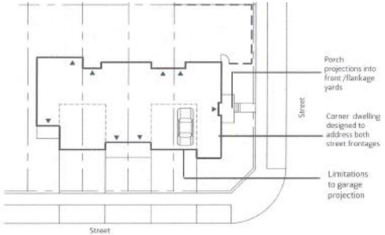
Conceptual siting of street townhouses
