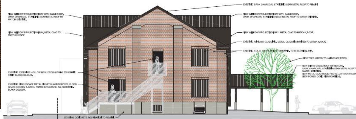
PROPOSED EXTERIOR ELEVATION - WEST
