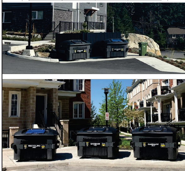
SAMPLE EARTHBIN CONTAINERS NO NEED FOR ENCLOSURE, REGULAR GARBAGE / RECYCLING TRUCK PICK-UP: FRONT LOAD
