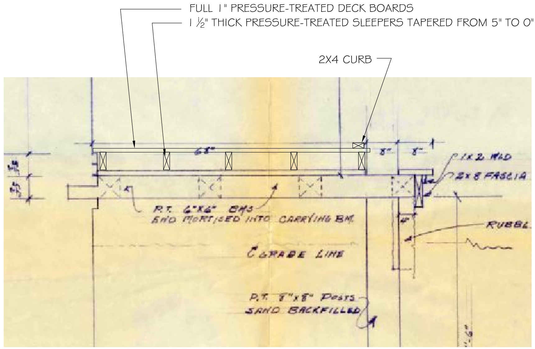
EXISTING PORCH SECTION WITH NEW OVERLAY
