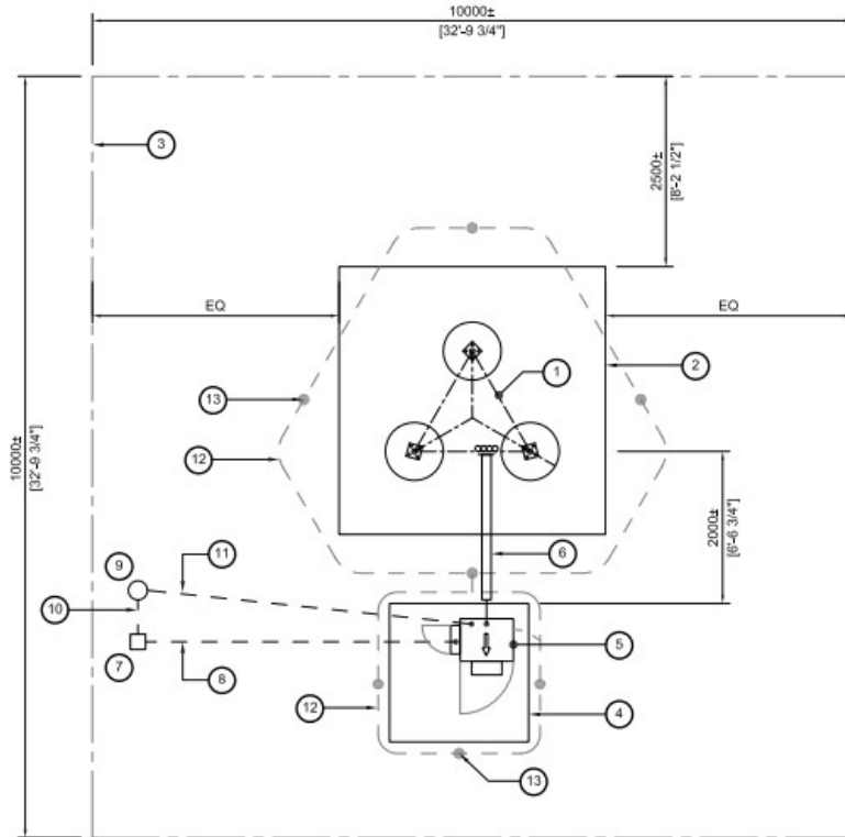
SITE LAYOUT & GROUNDING SCALE : NTS
