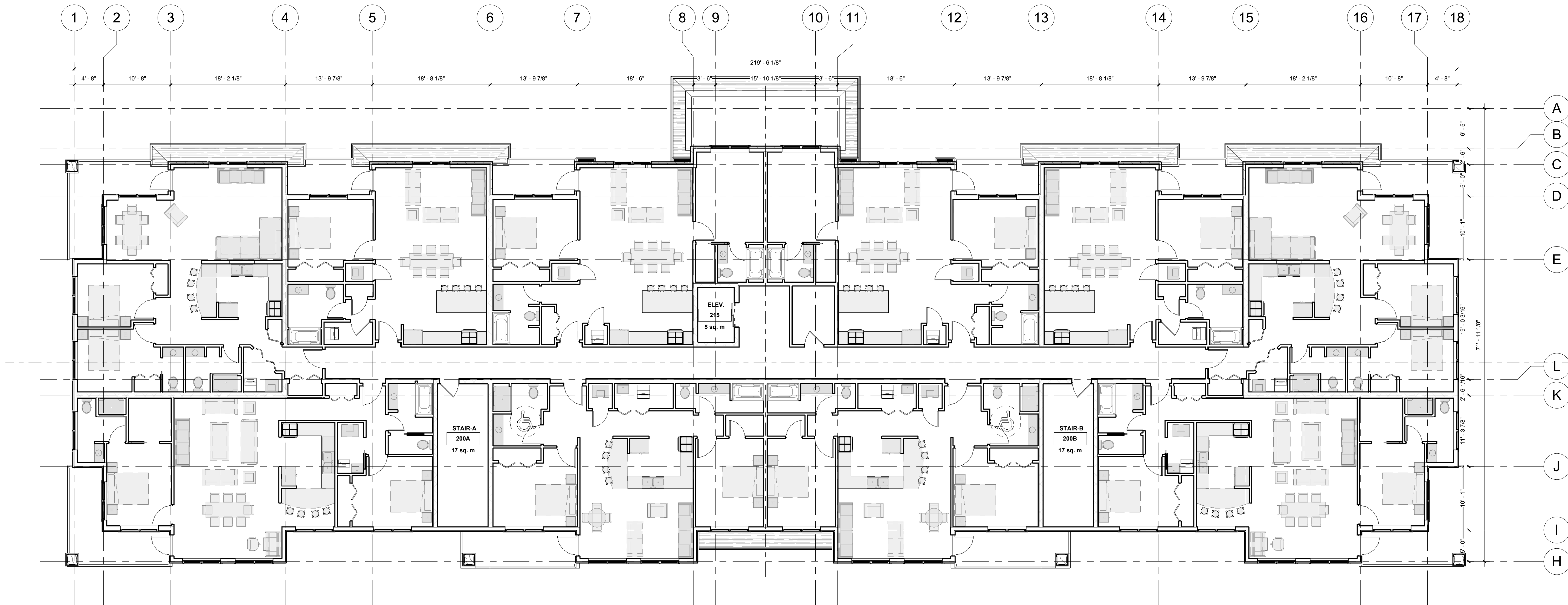
1 PROPOSED SECOND FLOOR LAYOUT 1 : 100
